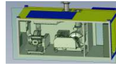
turbo blowers
